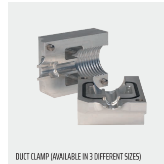
DUCT CLAMP (AVAILABLE IN 3 DIFFERENT SIZES)
